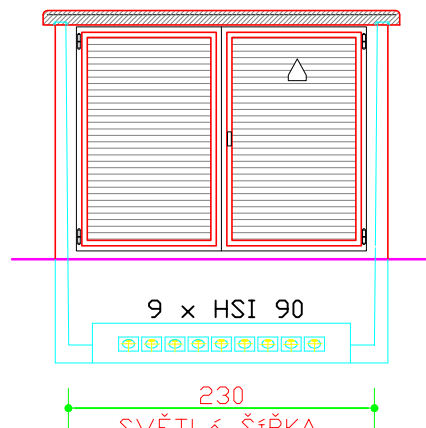
POHLED "C"
